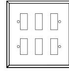
6 gang 146x146mm
